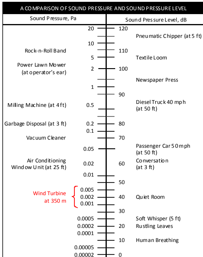
Figure 2. A comparison of sound pressure and sound pressure level (wind turbines in relation to other sources)
