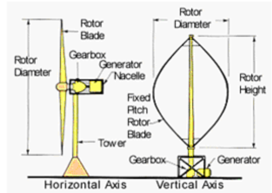
Figure 1. Typical Wind Turbine Configuration 1
