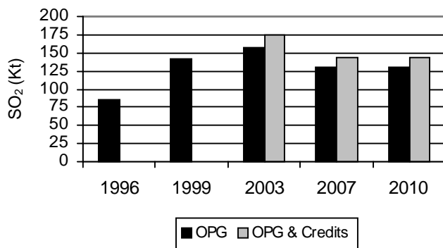
Figure 8: Sulphur Dioxide Emissions from Ontario's Electrical Sector, Past, Present & Projected
