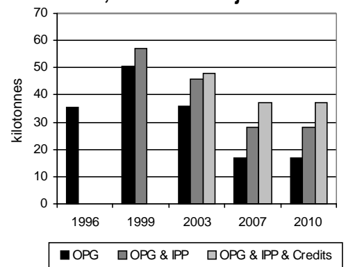
Figure 7: Nitrogen Oxide Emissions from Ontario's Electrical Sector, Past, Present & Projected
